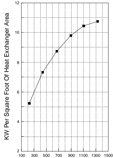
Figure 72A. Minimum air velocity required for ULTRA-SAFE™, feet per minute (meters per minute)
