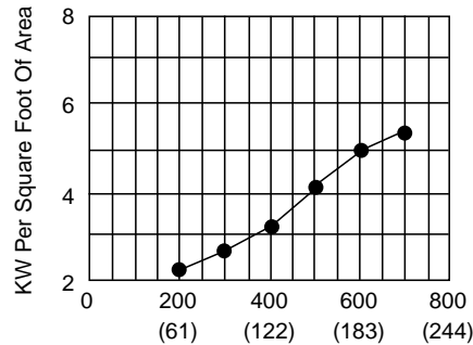
Figure 72B. Minimum air velocity required for EP2 feet per minute (meters per minute)
